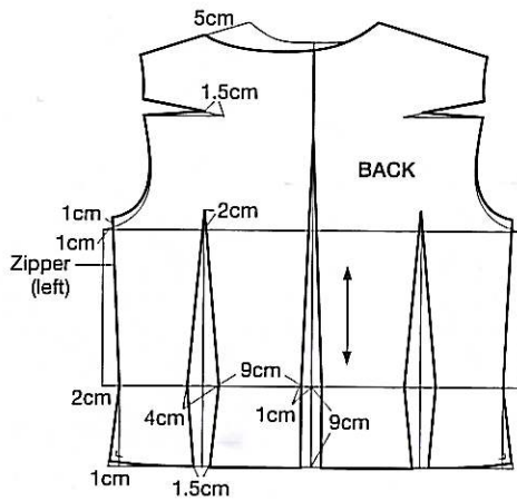
2 Draw the neckline on the bodice back with left and right asymmetry.
