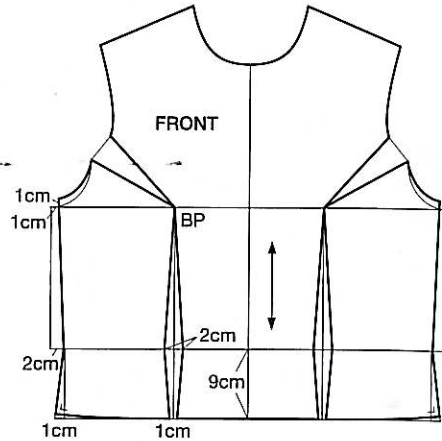
3 Draft a pattern for a fitted bodice front.
